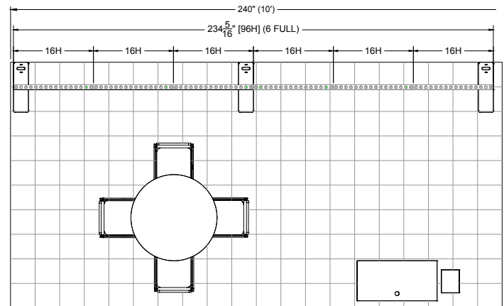
Electrical - Top View
